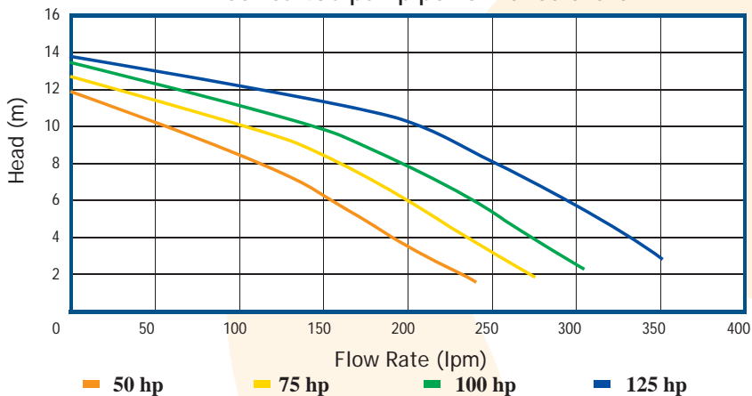
Series 40C pump performance chart
